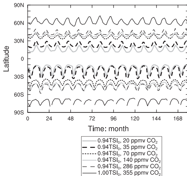
FIG. 4. Seasonal cycle of the sea ice margin, defined as the location where the sea ice fraction is equal to 50% in the central Pacific Ocean ( 160^\circ\text{E} – 160^\circ\text{W} ).
